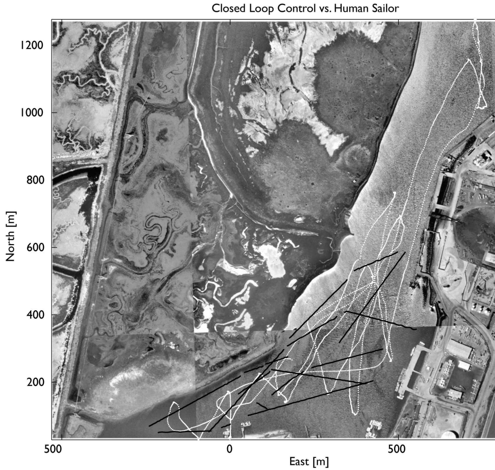
Fig. 15. Satellite photograph of harbor where the Atlantis was sailed under computer control. The white dots are data recorded from a human sailor using a conventional sloop rig. The black dots show the data from various closed loop computer controlled segments. Note how straight and “unnatural” they are. Simply, they do not look human.
