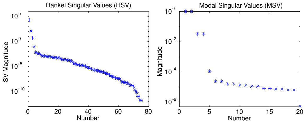
Fig. 11. The plot of the Hankel singular values of the system, showing that the experimental data is best represented by a 4th order system (left), and a singular value plot of the system modes showing again a large drop after 4 modes, again indicating that the system is 4th order (right).
