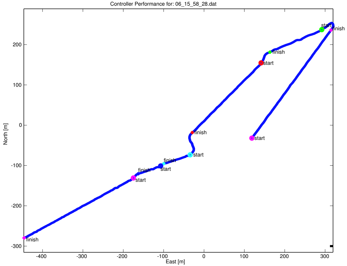
Fig. 16. Birds eye view of Atlantis under computer control, propelled by the wing-sail. Path regulation happens between each “start” and “end” pair, with the curves in between being performed open-loop with a feed-forward command.
