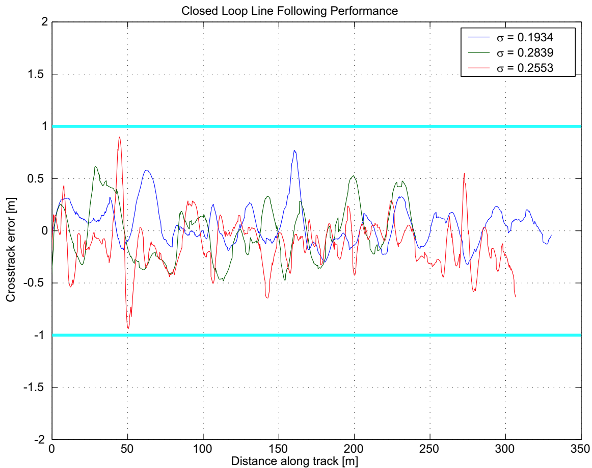
Fig. 18. Aggregate plot of computer controlled sailing passes, with lines at \pm 1 meter bounds, overlaid on top of one another. The differences in path length have to do with distance to shore, and the desire not to run aground. The controller keeps the Atlantis well within the one meter bound, and shows a standard deviation of less than 30 cm.
