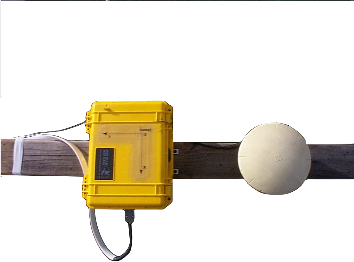
Fig. 3. The Atlantis uses a low-cost attitude solution that is based on a quaternion solution to Wahba's problem, where the two observed vectors are Earth's gravitation and magnetic fields. The solution produces 100 Hz. attitude data and is based on an Analog Devices 2-axis accelerometer and Honeywell 3-axis magnetometer.
