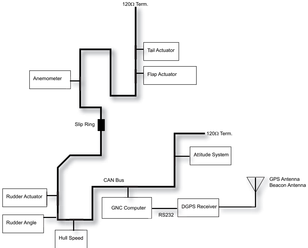
Fig. 2. Block diagram of the major subsystems of the Atlantis. Note that both power and CAN signals go through a slip ring at the top of the stub mast in order to electrically connect the rotating wing to the rest of the system.
