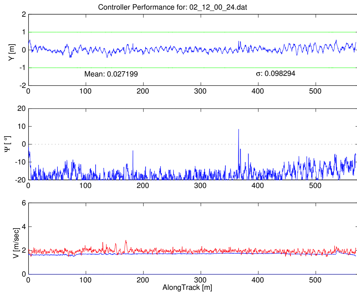
Fig. 14. Close up of the first section pictured in Figure 13, showing very precise control while under trolling motor propulsion and autonomous control. The mean of the path is less than 3 cm., and the standard deviation is less than 10 cm. Note that the presence of a current is indicated by a constant heading error (middle) as well as a mismatch between the GPS velocity and the hull speed sensors (bottom).
