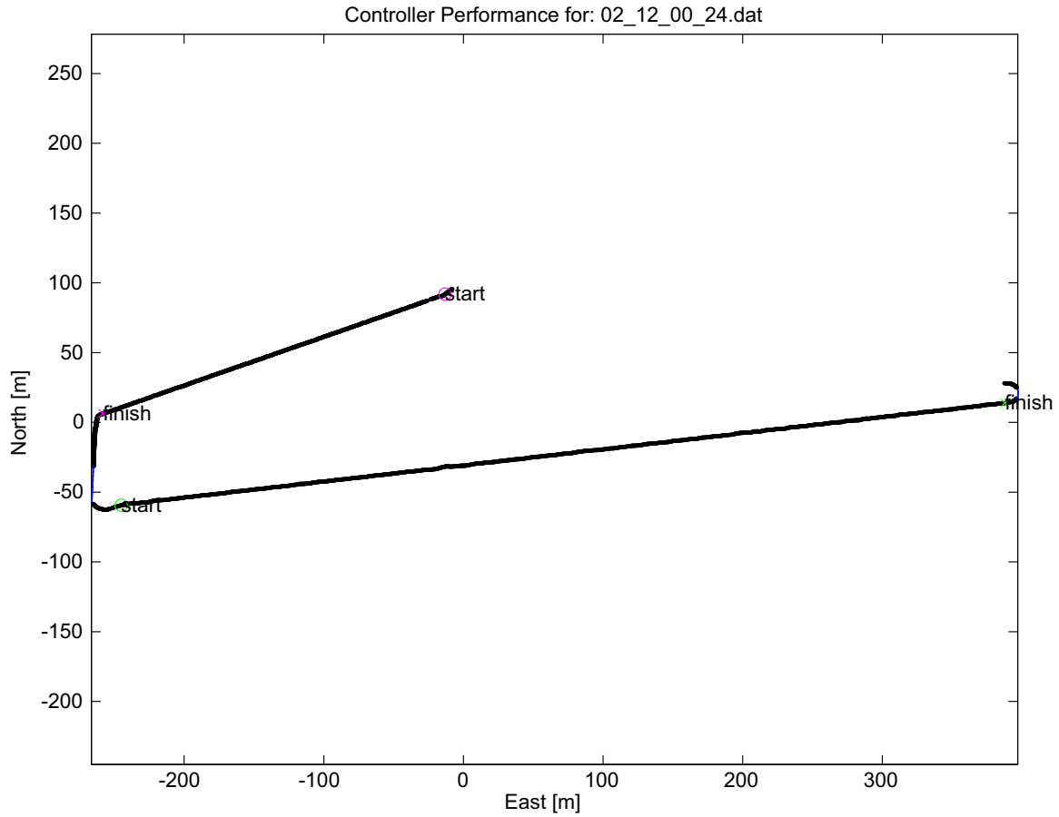
Fig. 13. The trajectory as recorded by the Ag122 Differential GPS receiver while under computer control. Note that feedback control is only used on the straight line segments. Turns are accomplished by open-loop feed-forward commands. To the resolution of this image, cross-track errors are less than one pixel wide.
